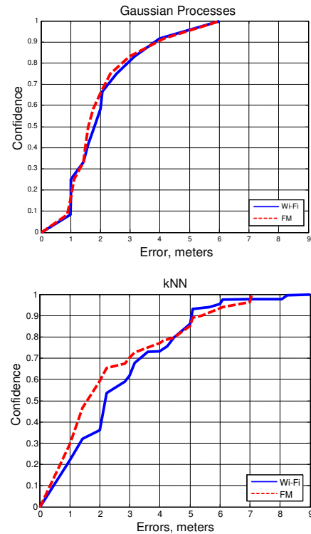
Fig.4. FM vs. Wi-Fi localization systems
